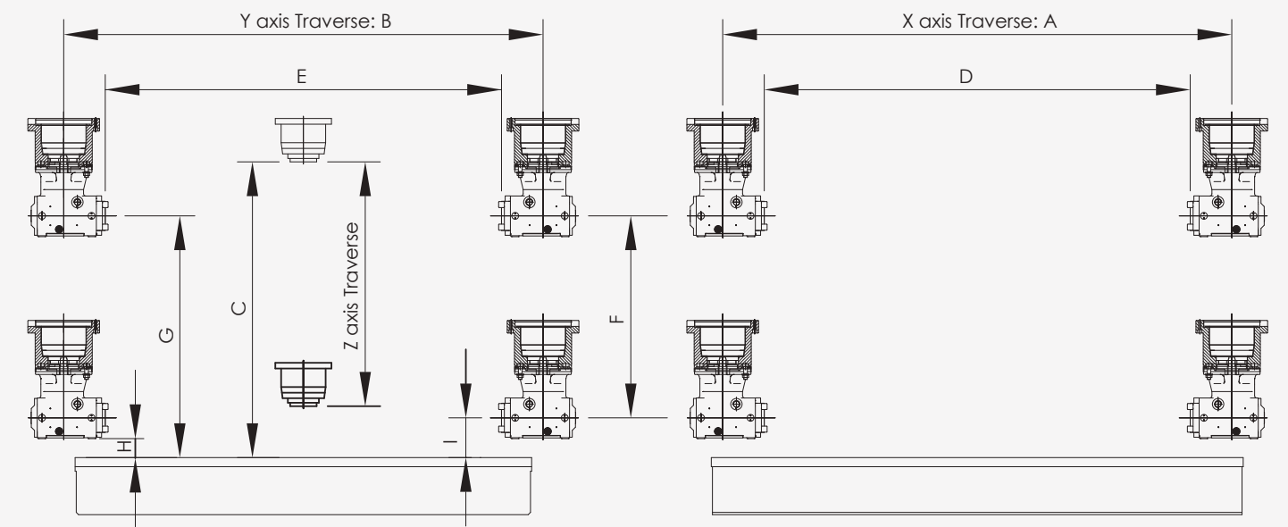
HF-M90L
