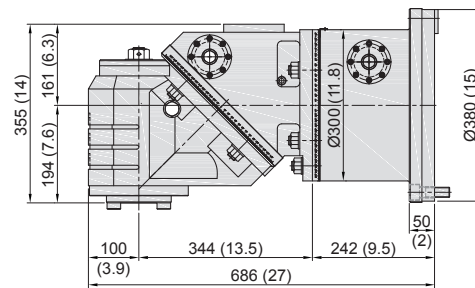
Universal Head Ø130 (Manual)
