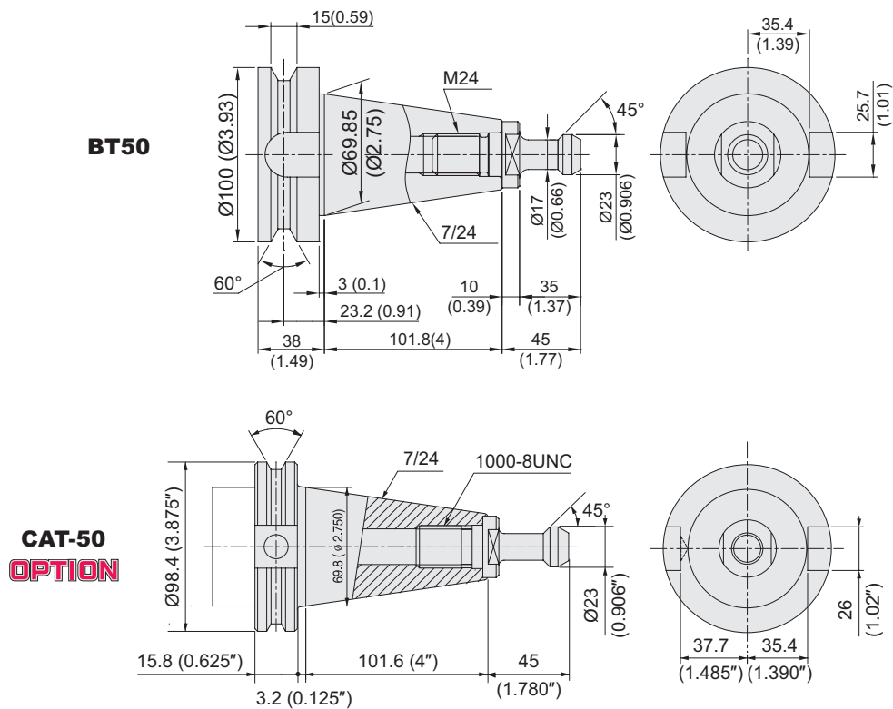
Tool Shank
