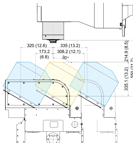
Tilting : A-axis +30°
