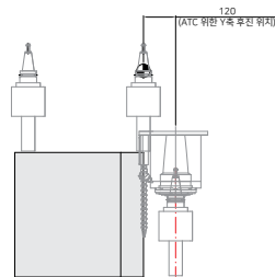
LEFT VIEW
