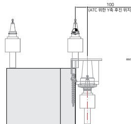
LEFT VIEW
