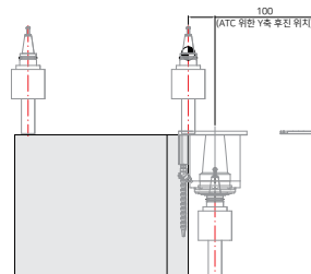
LEFT VIEW
