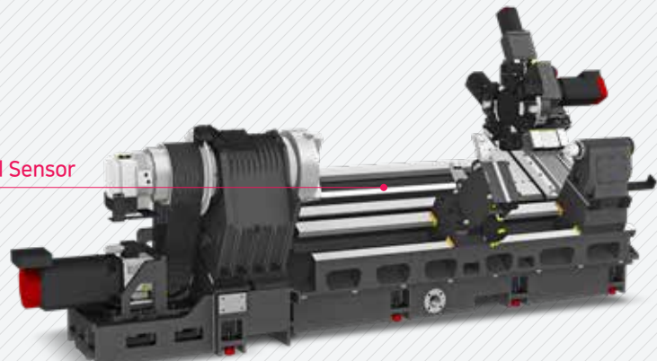
Structure thermal displacement error correction
