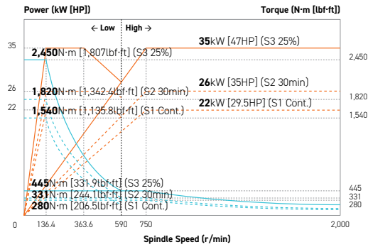
L4000M/LM 2,000 rpm
