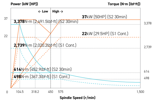
L4000MC/LMC 1,500 rpm
