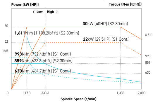
L4000/M/L/LM 2,000 rpm
