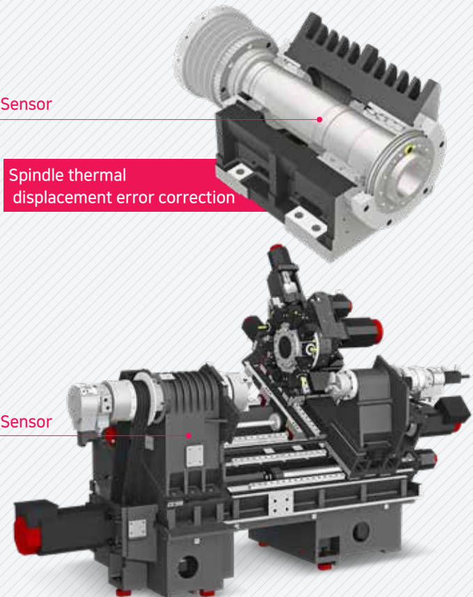
Structure thermal displacement error correction
